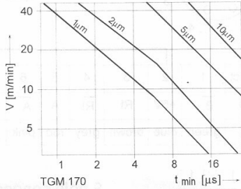
Maximum operating speed diagram.
