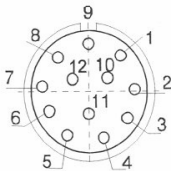
12 pole connector (Contact) sine-wave voltage 1Vpp signals (SV)
